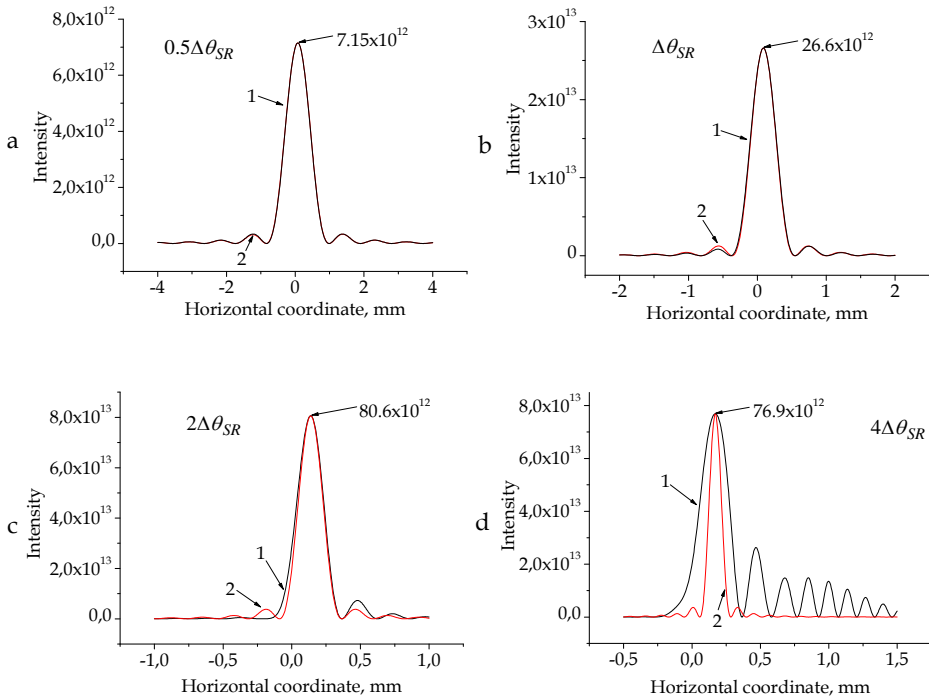
Fig. 10. Intensity distributions (photons/s/mm 2 /(0.1% bandwidth)) in the median plane of the focused synchrotron radiation for different horizontal angular aperture \theta_{lens} of the lens: a - \theta_{lens} = 0.5\Delta\theta_{SR} , b - \theta_{lens} = \Delta\theta_{SR} , c - \theta_{lens} = 2\Delta\theta_{SR} and d - \theta_{lens} = 4\Delta\theta_{SR} . Curve 1 - focused synchrotron radiation, curve 2 - approximation by (\sin(\xi)/\xi)^2 , see Eq. (5).
