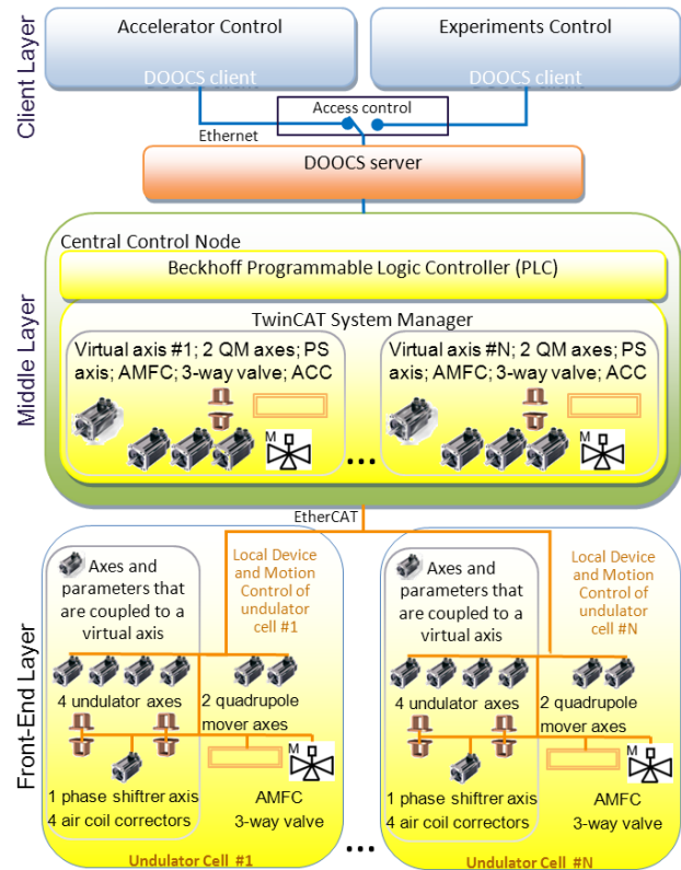
Figure 3: Schematic overview of the undulator control system.
