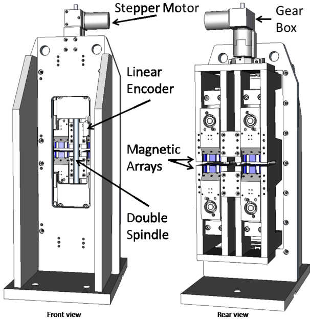
Figure 5: Motion control components of the phase shifter
