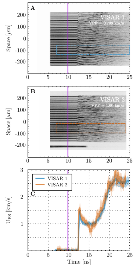
FIG. 13. Analysis of the VISAR data collected from a 100 \mu\text{m} -thick Si single crystal shock-compressed using a 10 \text{ ns} , 29 \text{ J} square pulse generated by the DiPOLE-100X laser system and focused on the target using a 500 \mu\text{m} diameter phase plate. The velocimetry data (c) show the free surface velocity ( U_{FS} ) for each VISAR (blue and orange lines) with the shaded area corresponding to the 1\sigma uncertainty. The corresponding corrected VISAR 2D-images are shown in (a) and (b). The vertical purple line indicates the probing time by the x-ray beam. In all images, the DiPOLE-100X laser pulse arrives at 0 \text{ ns} . The dashed rectangles in (a) and (b) correspond to the region of interest used to obtain the velocity traces in (c).
