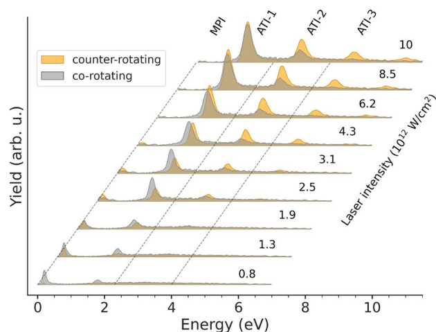
Fig. 3. Photoelectron spectra for different peak intensities of the optical laser for co- (darker shade) and counter-rotating (lighter shade) polarized NIR laser pulses. The zero lines for each peak intensity (indicated in multiples of 10^{12} \text{ W/cm}^2 on the right) have been offset to make the individual results visible.
