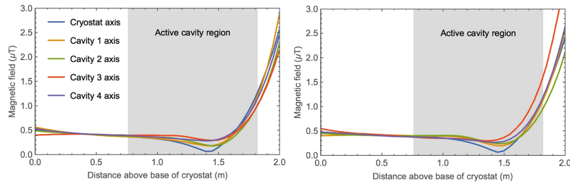
FIG. 3. Magnetic field distribution inside the cryostat XATC1 (left) and XATC2 (right) along the different axes.
