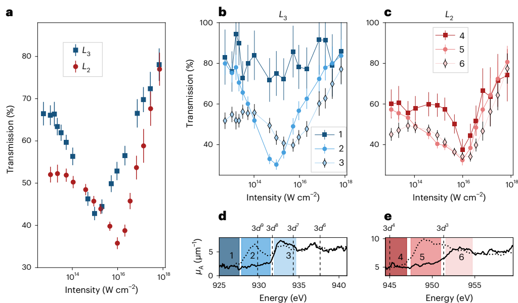
Fig. 2 | Transition from RSA to SA. a , Transmission of an XFEL pulse centered at the L_2 and L_3 edges of a 100-nm-thick Cu foil as a function of pulse intensity I . In both cases, the transmission first decreases (RSA), reaches a minimum and then increases (SA) as a function of intensity. b, c , Transmission at the L_3 edge ( b ) and L_2 edge ( c ) in selected spectral regions below the L_3 or L_2 pre-edge (1, 4), on the L_3 or L_2 pre-edge (2, 5) and on the L_3 or L_2 edge (3, 6), respectively, as shown
