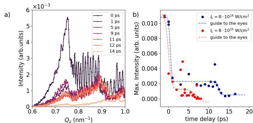
Figure 3. In-plane signal along Q_z around the dynamical diffraction area between 0.6 and 1.0 \text{ nm}^{-1} . (a) In-plane signal for different time delays at lower laser intensity case ( 8 \times 10^{14} \text{ W/cm}^2 ). (b) The circular dots display the integrated signal between Q_z = 0.65\text{--}0.79 \text{ nm}^{-1} as a function of time delay. The dashed line represents a guide to the eyes. Blue color stands for the lower laser intensity of 8 \times 10^{14} \text{ W/cm}^2 and red denote the higher laser intensity 8 \times 10^{15} \text{ W/cm}^2 .
