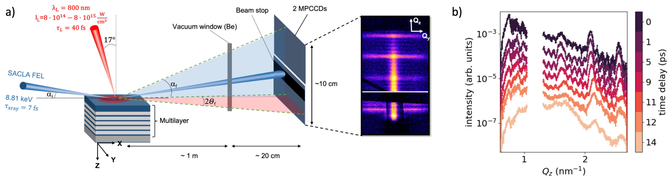
Figure 1. Schematics of the experimental setup to investigate the surface and subsurface solid-density plasma dynamics with GISAXS using single femtosecond X-ray FEL pulses. (a) An ML sample consists of 5 repetitions of tantalum (Ta) and copper nitride (Cu 3 N) of 4.5 and 8.5 nm thickness covered by a 200 nm aluminium capping layer. The samples were irradiated by an optical laser with a central wavelength of 800 nm, intensity of (8 \pm 0.2) \times 10^{14} or (8 \pm 0.2) \times 10^{15} W/cm 2 with 40 fs pulse duration. The laser is irradiated by an incident angle of 17° from the surface normal in p polarization. The X-ray pulses with 8.81 keV photon energy, 7 fs FWHM duration are irradiated on the sample at the grazing-incidence angle of \alpha_i = 0.75^\circ , i.e., slightly above the critical angle of external total reflection of the layer materials. The laser beam is defocused to obtain a \sim 500 \mu\text{m} spot diameter to cover the X-ray footprint of \sim 300 \mu\text{m} at the surface. Scattered photons are recorded by 2 modules of the MPCCD area detector placed around the specular direction. The strong specular peak at Q_z = 1.16 nm -1 is blocked. (b) In-plane signal along Q_z (at Q_y = 0 ) for different time delays between 0 and 14 ps after the laser intensity peak.
