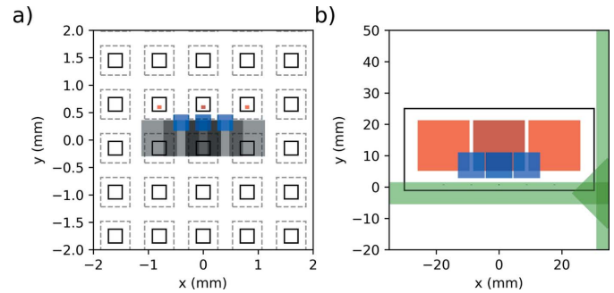
Figure 3 BOZ calculator showing the beams at (a) the sample and (b) the detector planes. The focused 1st zone-plate order beam footprint at the respective positions is shown as red for the fundamental and blue for the second harmonic. The 0th zone plate order is shown as gray. Individual membrane windows and the etching lines are shown in (a) as continuous and dashed lines, respectively. In (b) the DSSC sensor is represented by the black rectangle and the DSSC filter mount is represented by the green shapes.
