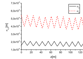
Figure 2: Evolution of the horizontal and vertical dimensions of the electron bunch as a function of the distance inside the SASE3 undulator. The plots refer to the longitudinal position inside the bunch corresponding to the maximum current value.
