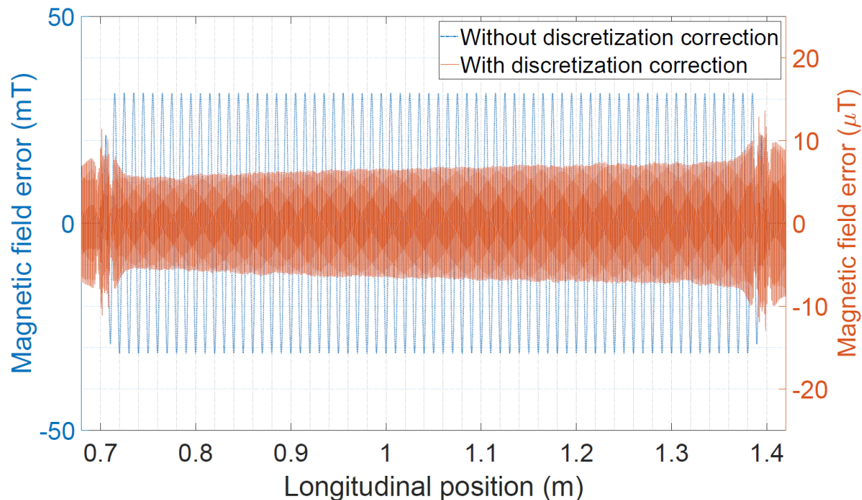
Magnetic field error comparison for the case where the discretization effect is corrected (orange) and is not corrected (blue)
