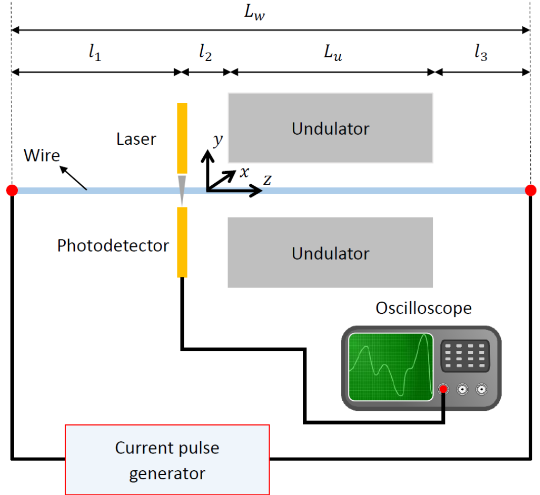
Two-dimensional scheme of the pulsed wire system and main lengths
