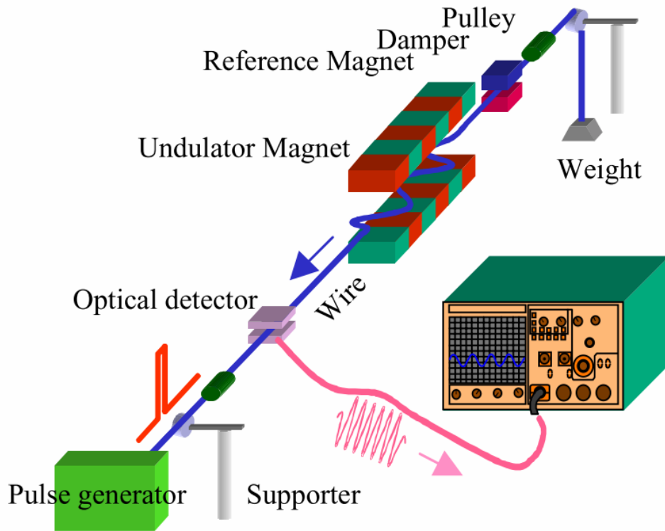
Simplified diagram of the pulsed wire system [1]
