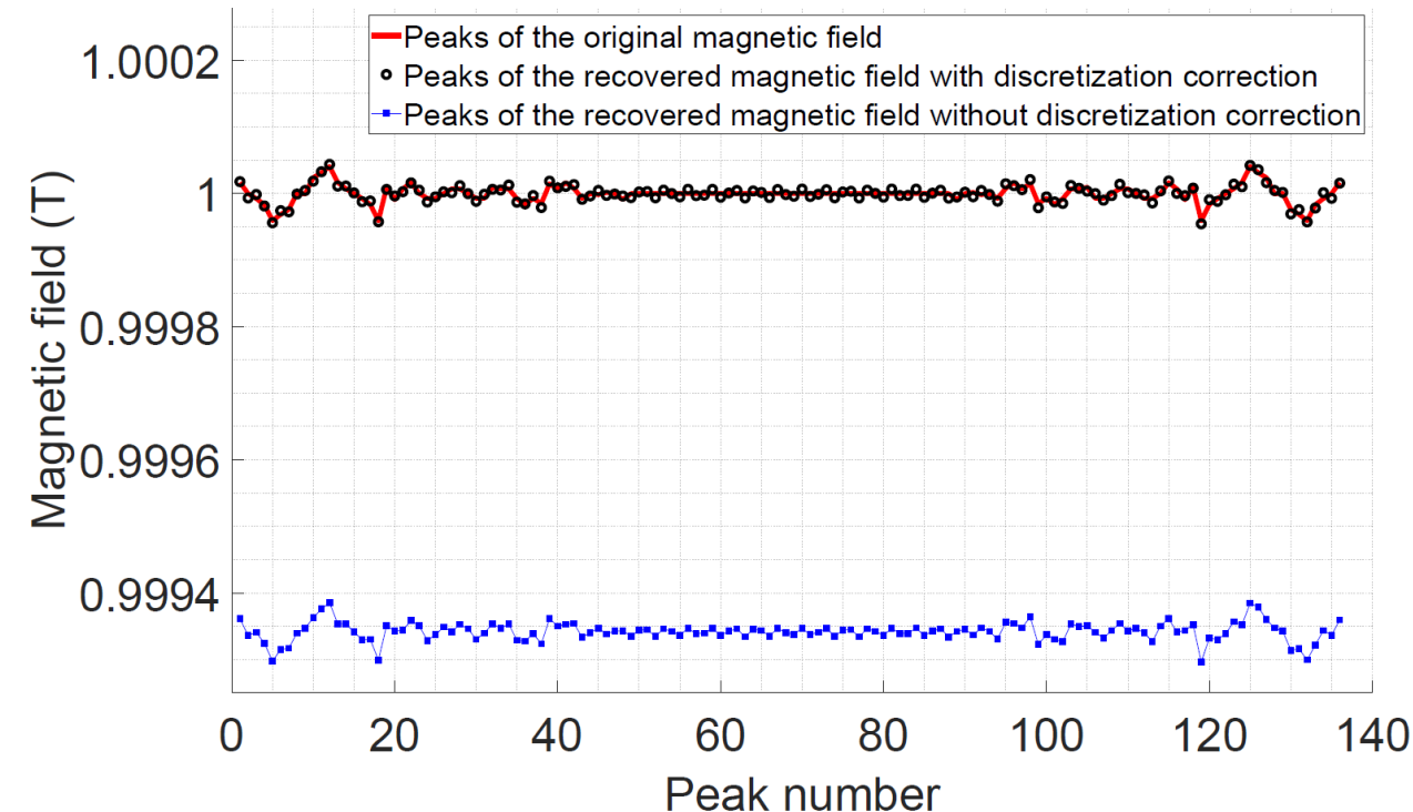
Comparison among the peaks of the original magnetic field (red line), recovered with (black circles) and without discretization correction (blue squares)
