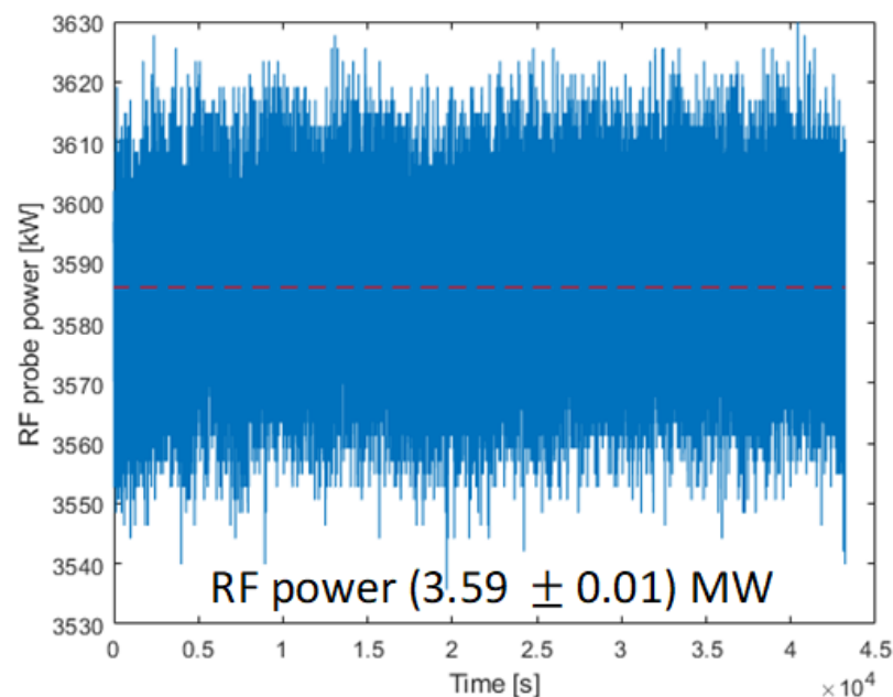
Figure 3. Stability measurement of the RF probe power in the ARES gun over 12 h.
