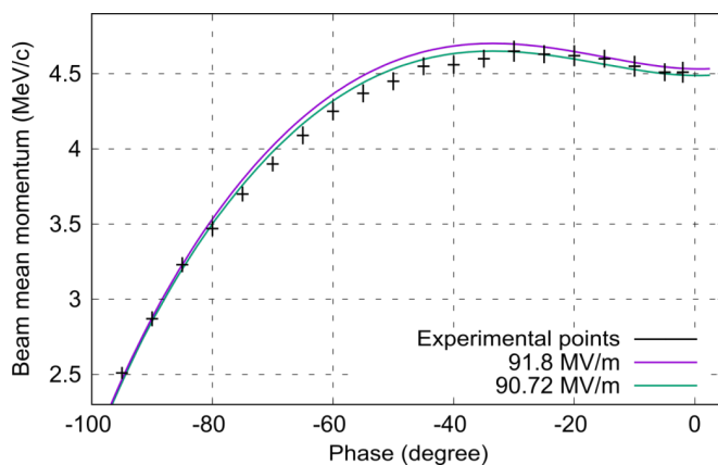
Figure 8. Measured beam momentum vs. RF phase. The acceleration gradient is estimated with around 91 MV/m from fitting ASTRA simulations.
