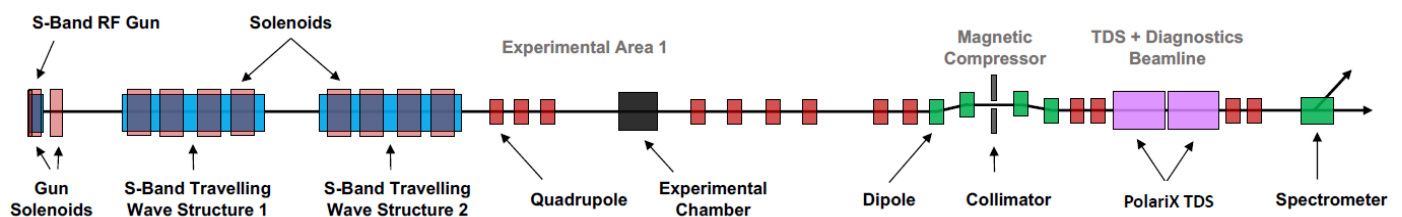
Figure 1. Future layout of the ARES linac at SINBAD.
