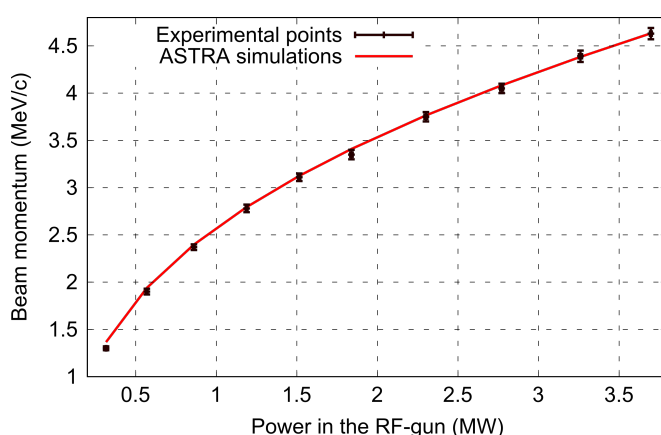
Figure 7. Measured beam momentum vs. RF power. The momentum measurement was done using the first vertical corrector magnet. The RF phase was fixed at -20 deg relative to zero-crossing. The measurement points are compared with ASTRA simulations.
