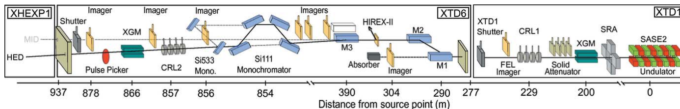
Figure 5 Beam transport in the XTD1 and XTD6 underground tunnels up to the XFEL Headquarters EXPERIMENT hall 1 (XHEXP1). The X-rays enter from the right. Not all components are shown. A detailed list of devices and distances can be found in Appendix B.
