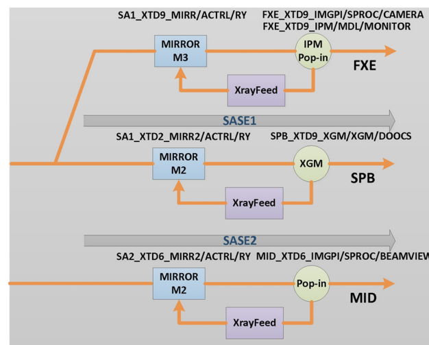
Figure 3: Block diagram of actuators and diagnostic devices taking part in feedback setups. Setups of three instrument lines are shown – SPB, FXE and MID.
