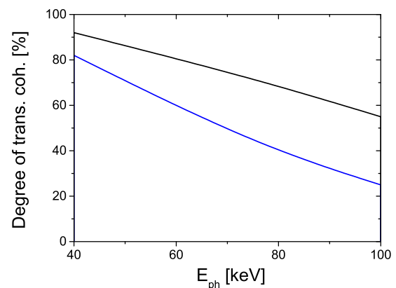
Figure 4: Expected degree of transverse coherence (see the definition in [16]) of SASE FEL radiation as a function of photon energy. Blue line: normalized emittance is 0.3 mm mrad. Black line: normalized emittance is 0.2 mm mrad. Electron beam energy is 17.5 GeV. Estimates were done using the results of Ref. [16].
