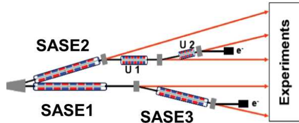
Figure 1: Layout of the European XFEL undulator tunnels.
