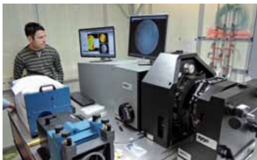
Figure 3 Setup of the Fizeau interferometer in the PETRA III laboratory at DESY
