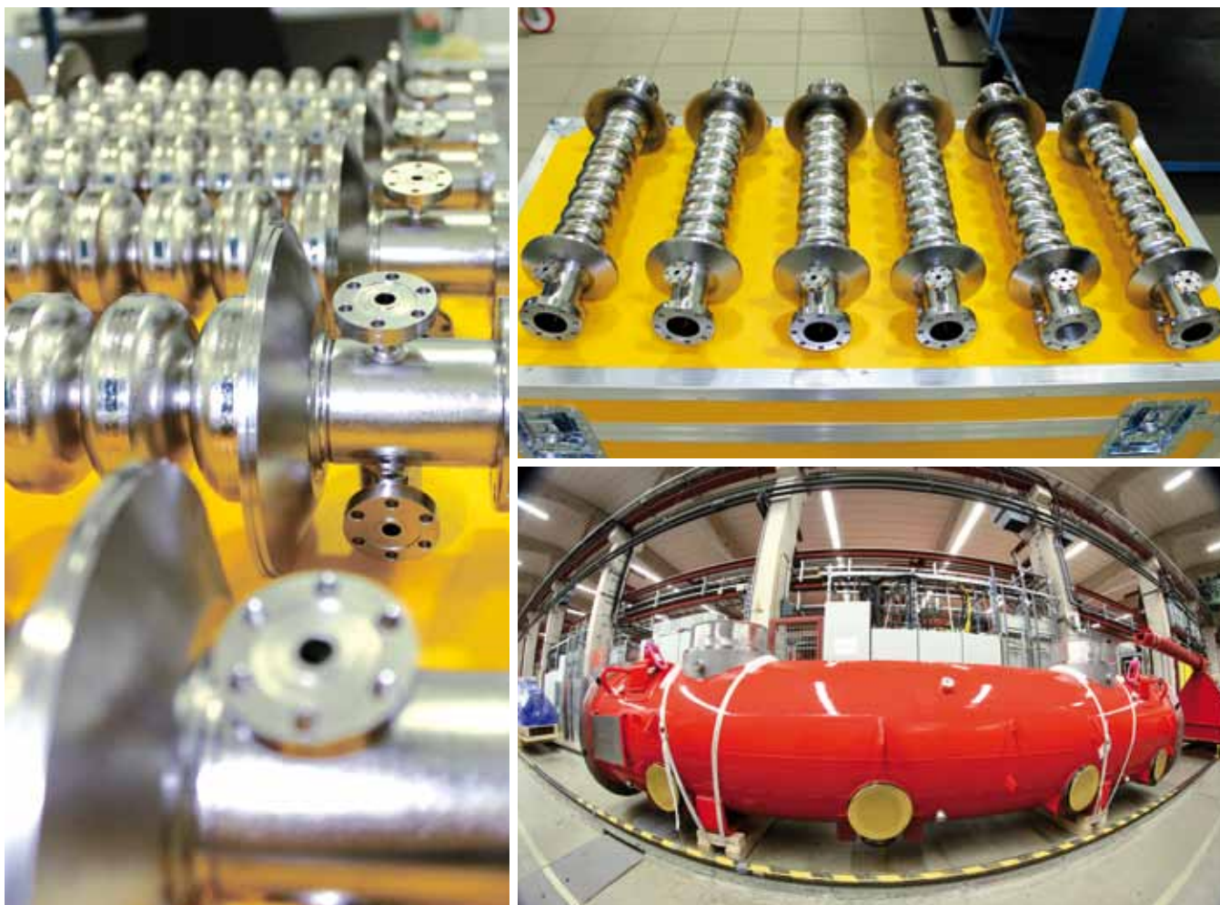
Figure 8 3.9 GHz system. The linearization of the RF-induced curvature in phase space is necessary to preserve the beam quality in the subsequent bunch compressor stages before entering the main linear accelerator. The RF curvature linearization is achieved by a third-harmonic section after the RF gun. The single module at 3.9 GHz consists of eight superconducting RF cavities (IKC IT03/WP46 by INFN – Sezione di Milano, Laboratorio Acceleratori e Superconduttività Applicata (LASA), Italy).
