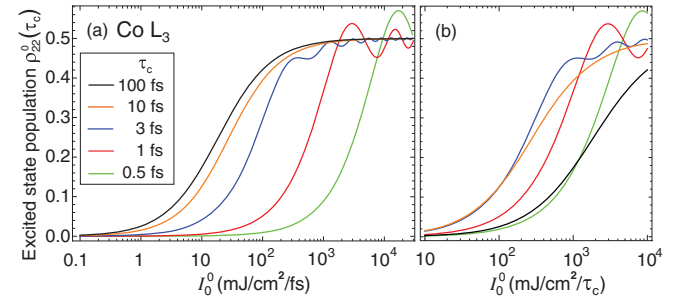
FIG. 2 (color). (a) \tilde{\rho}_{22}^q(\tau_c) as a function of linearly polarized incident intensity I_0^q for different coherence times \tau_c of the incident pulses for the L_3 edge of a 20 nm thick Co metal film. We assumed resonance excitation, \hbar\omega = \mathcal{E}_0 , and experimental peak cross sections as discussed in the text. (b) Same as in (a) as a function of the incident fluence per coherence time of the pulse.
