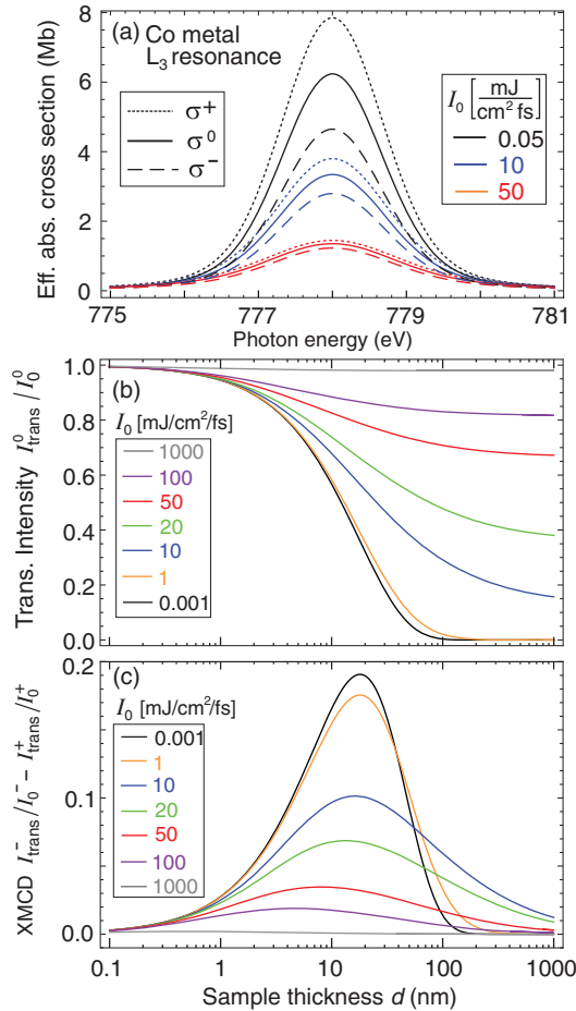
FIG. 3 (color). (a) Change of the effective polarization dependent absorption cross section 2\lambda(f''_0^q + 2f''_{\text{NL}}^q) for the L_3 resonance in Co metal for three incident intensity values, assuming alignment of the x-ray propagation direction with the film magnetization and the long coherence time limit, Eq. (9). The low intensity cross sections shown as black curves are nearly identical to the spontaneous ones shown in red in Fig. 1. (b) Dependence of the transmission contrast as a function of sample thickness and incident intensity for resonant L_3 excitation of a Co metal film due to charge absorption with linearly polarized light, according to Eq. (7). (c) Same as (b) for the transmitted XMCD contrast.
