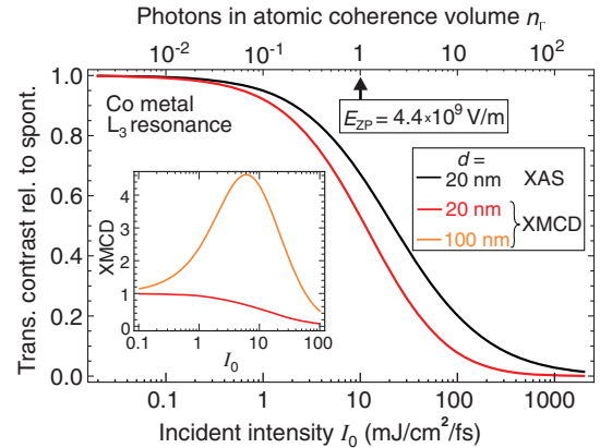
FIG. 4 (color). Dependence of the transmitted intensity according to Eq. (7) and Eq. (9) in the presence versus absence of stimulation for a 20 nm Co metal film as a function of incident intensity. The black curve represents the linear polarization or charge response [I_{\text{trans}}^0]_{\text{stim}}/[I_{\text{trans}}^0]_{\text{spont}} and the red curve is the transmitted XMCD difference intensity [I_{\text{trans}}^- - I_{\text{trans}}^+]_{\text{stim}}/[I_{\text{trans}}^- - I_{\text{trans}}^+]_{\text{spont}} . The top scale is discussed in the text. The inset shows the relative transmitted XMCD contrast for film thicknesses of 20 nm (red) and 100 nm (orange) as a function of incident intensity.
