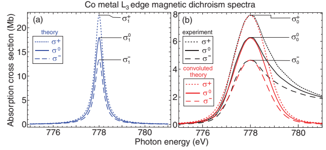
FIG. 1 (color). (a) Polarization and photon energy dependent L_3 absorption cross sections \sigma_{\text{abs}}^q = 2\lambda f''^q for Co metal, calculated by use of Eq. (2) and the parameters \Gamma and \Gamma_x^q in Table I. (b) Comparison of the experimental dichroic cross sections (black lines) and the theoretical cross sections in (a) convoluted with a Gaussian of 1.4 eV FWHM. Note that the corresponding blue and red curves have the same areas, but their peak values differ by a factor of \sigma_1^q/\sigma_0^q = 2.9 .
