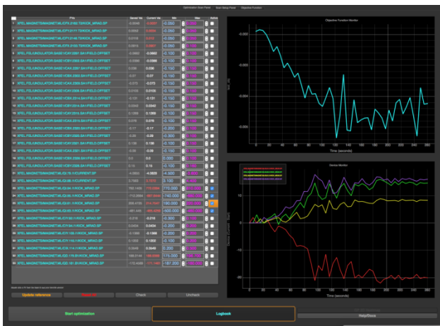
Figure 5: SASE tuning with 4 quads in the injector dogleg section. SASE level increased from 100 \mu J to 240 \mu J.
