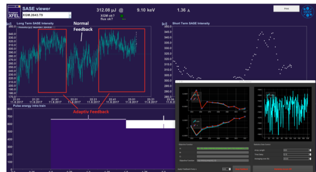
Figure 7: Example of adaptive feedback during European XFEL operation. Lower right corner shows the GUI featuring the current reference and measured orbit, and the photon pulse energy monitor.
