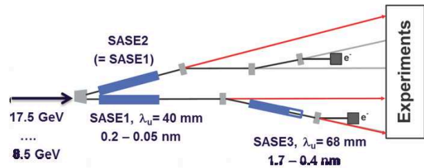
Figure 1: Schematic layout of the European XFEL beam distribution
