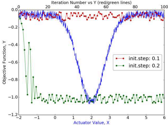
Figure 2: Objective function vs. actuator (blue curve, lower axis). Objective function vs. iteration number for different initial steps (red and green curves, upper axis).
