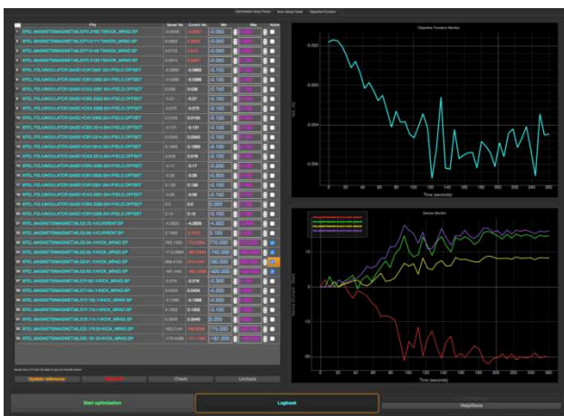
Figure 5: SASE tuning with 4 quads in the injector dogleg section. SASE level increased from 100 \mu\text{J} to 240 \mu\text{J} .
