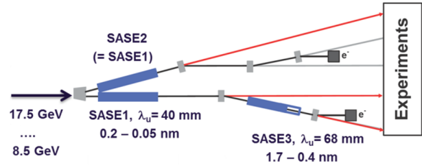
Figure 1: Schematic layout of the European XFEL beam distribution.
