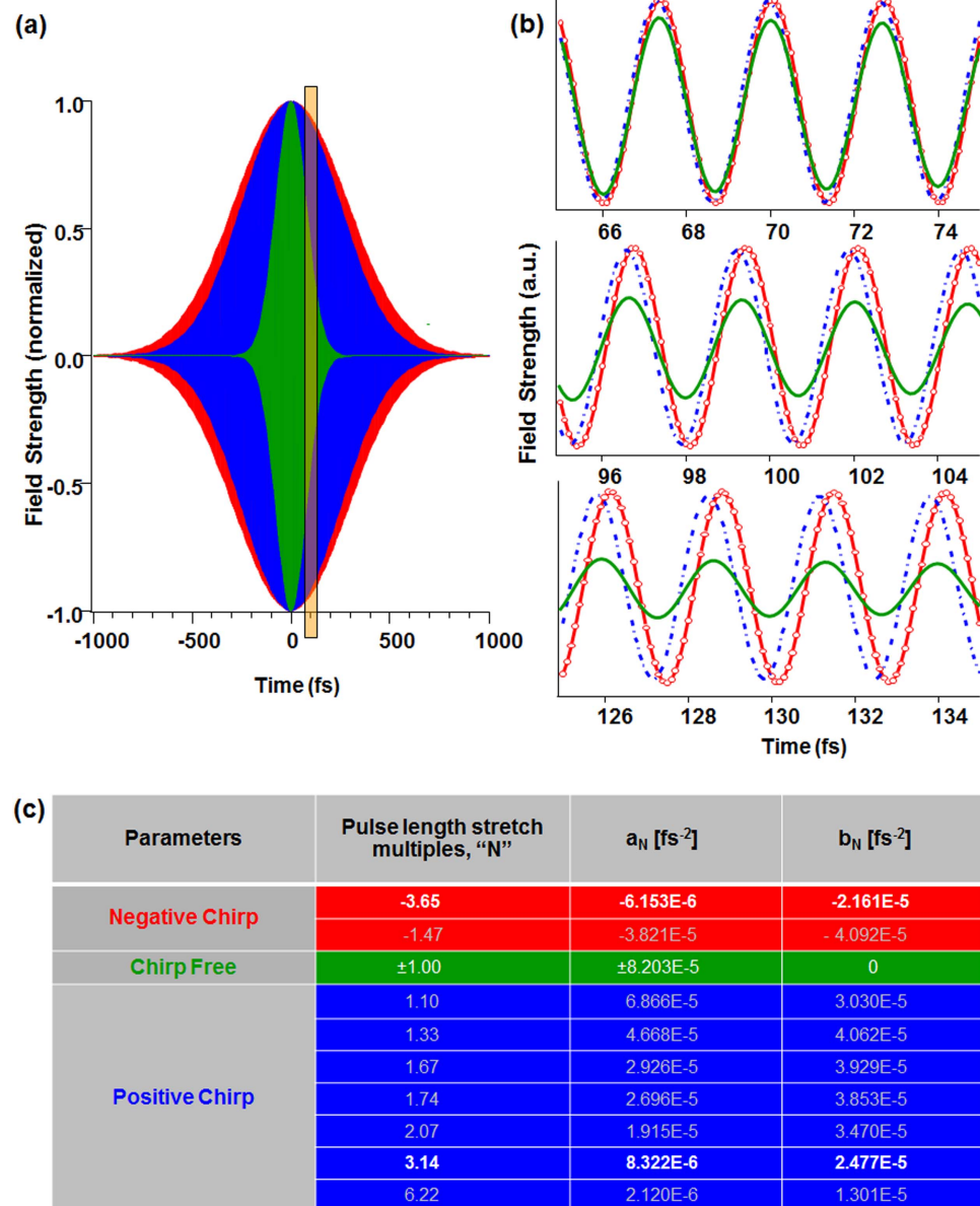
Figure 6. (a) The simulated driving pulse waveforms (normalized) for TL pulse duration of 130 fs (green), negative chirp pulse duration of -475 fs (red), and positive chirp pulse duration of 408 fs (blue) used in the experiment. The vertically semi-transparent bar area across the three wave-packets represents a time-window of (65, 135) fs with respect to the field peak. (b) 'Zoomed-in' views for three typical '10-fs' sub-windows within the '65–135 fs' window (the central time scales of the three sub-windows are 70, 100, 130 fs with respect to the field peak) and comparison of the electric fields of the three normalized pulses, demonstrate the phases of negative (red circle-line) and positive (blue dot-line) chirp pulses are shifting oppositely respected to the chirp-free pulse (green solid-line). (c) Parameters for various chirp pulses used in the experiment, and in part (a) ' -475 fs' corresponds to ' N = -3.65 ', and ' 408 fs' corresponds to ' N = 3.14 ' in the table.
