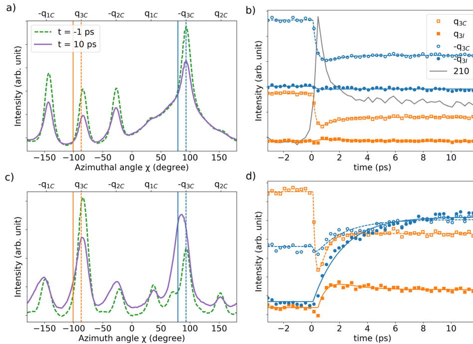
FIG. 4. (a) Intensity profile of the 6 first order CDW satellites around the 100 Bragg peak for a negative delay at t = -1 ps in dashed green line and a positive delay at t = 10 ps in a continuous purple line. The vertical dashed blue (orange) line indicates the position in the commensurate phase of the -q_3 ( q_3 ) satellite -q_{3C} ( q_{3C} ), while the continuous blue (orange) line indicates the position for the incommensurate phase of -q_3 ( q_3 ) satellite -q_{3I} ( q_{3I} ). (b) Time evolution after laser excitation of the CDW satellites intensity at the commensurate (open symbols, dashed lines) and incommensurate position (filled symbols, continuous lines) for the q_3 (orange) and -q_3 (blue) satellites, where the lines correspond to a fit of the data points with a two exponential time constants. The grey data point are the 210 Bragg peak intensity at l = 0 . (c) and (d) are for the 200 Bragg peak. In all figures, the sample temperature is T = 140 K, the laser fluence is F = 3.0 mJ/cm 2 and the incidence angle is \theta = 5^\circ .
