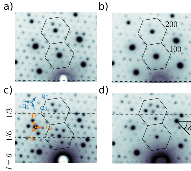
FIG. 2. Part of the electron diffraction pattern recorded at normal incidence (a) in the commensurate phase at T = 150 K and (b) in the nearly commensurate phase at T = 300 K, as well as for the case of a tilt angle of \theta = 5^\circ from normal incidence at (c) T = 150 K and (d) T = 300 K. The first Brillouin zones around the 100 and 200 Bragg peaks are shown as the hexagons. The 3 positive first order satellites q_1 , q_2 , and q_3 are shown as orange arrows, while the 3 negative satellites of the CDW -q_1 , -q_2 , and -q_3 are shown as blue arrows. For the tilted case, dashed lines at l = 0 , 1/6 , and 1/3 are shown. In (d), the azimuth angle \chi is shown. In all cases, the data are shown on a logarithm scale.
