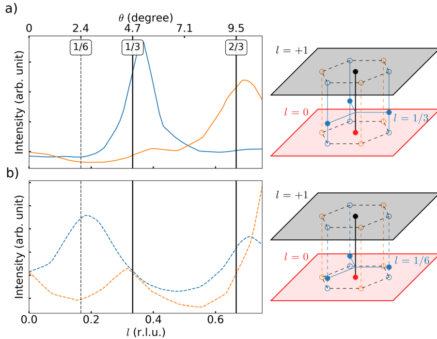
FIG. 3. Averaged intensity of the 3 positive CDW satellites in orange and 3 negative satellites in blue as function of the Miller index l and corresponding incidence angle \theta for the 200 Bragg peak, for (a) the nearly commensurate phase at T = 300 K and for (b) the commensurate phase at T = 150 K, together with a schematic in each case of the CDW in reciprocal space with the filled blue satellites at either l = 1/3 or l = 1/6 for the nearly commensurate or commensurate phase, respectively. The open orange and blue satellite circles are the projection on the l = 0 and 1 plane which are seen at normal incidence.
