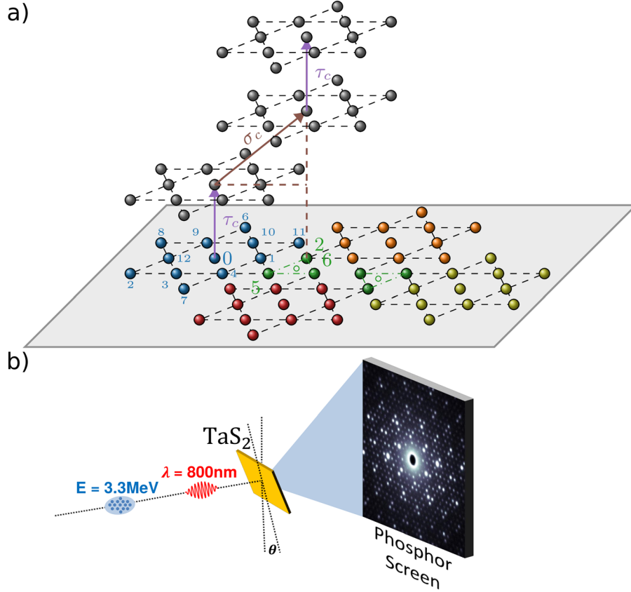
FIG. 1. (a) Direct space view of the star of David formation in the basal plane, where the 13 Ta atoms are numbered in sequence. The out-of-plane layer stacking for the commensurate phase is a succession of a \tau_c translation, positioning the star of David on top of each other in position 0, followed by a random selection between 3 possible \sigma_c translations positioning the star of David on top of positions 2, 5, or 6. In the nearly commensurate or incommensurate phase, the \langle\sigma_{h2}\rangle or \langle\sigma_1\rangle stacking, respectively, is a three times repeat of a translation linking the center of a star of David and the center of the 2-5-6 green triangle. After three such translations, the layer is back in the 0 position. (b) Schematic of the time-resolved electron diffraction experiment, where the sample is tilted by an angle \theta from normal incidence to probe the out-of-plane layer stacking changes between the commensurate and nearly commensurate or incommensurate phase. The 800 nm wavelength 50 fs laser pulse excites the TaS 2 sample. After a delay t , the 3.3 MeV 100 fs electron bunch diffracts from the sample on a phosphor screen.
