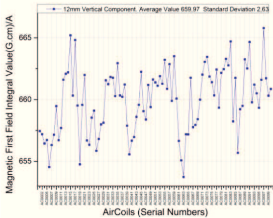
Figure 5: First field integral in Y direction at Y, Z=0 of entire amount of air coils with 12 mm gap. The ambient magnetic field is subtracted.
