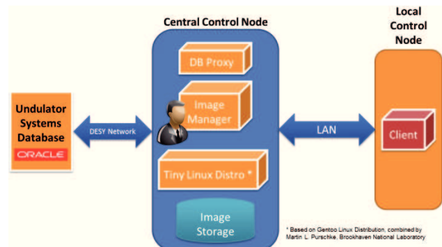
Figure 2: Schematic layout of the components of IDA.
