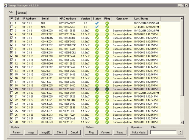
Figure 3: Main user interface of the IDA.
