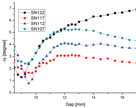
Figure 5: Measured optical phase jitter vs undulator gap. The optical phase jitter is minimum at the tuning gap and increases as gap is deviated from the tuning gap. For clarity, only 4 undulators among 20 are shown.
