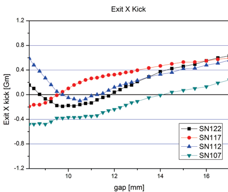
Figure 6: Required exit x-kicks for horizontal plane. For clarity, only 4 undulators among 20 are shown.
