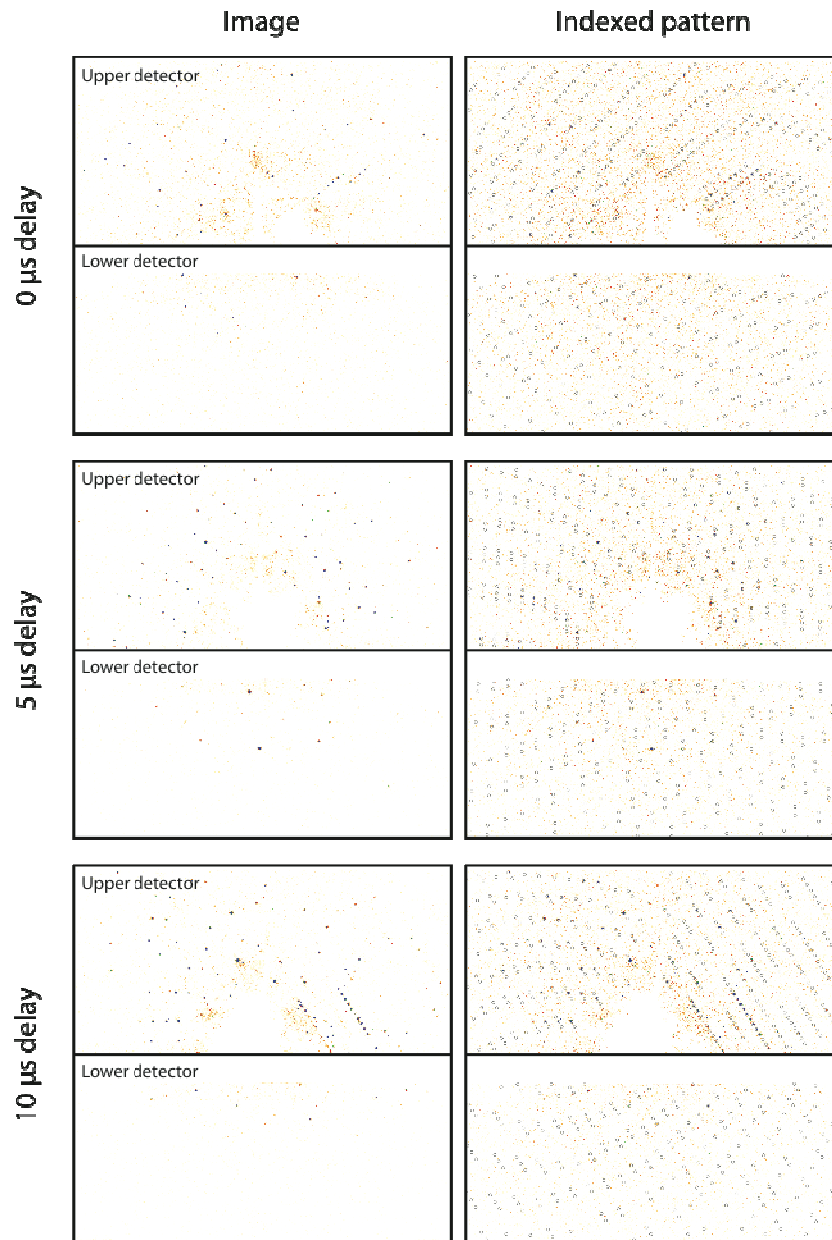
Fig. 2. Single-shot, single crystal diffraction patterns, from the pnCCD detectors, of PSI-fd (top) in the dark state, (middle) in the 5 \mu s pumped state, and (bottom) the 10 \mu s pumped state. The images on the right side are the same as the corresponding left side image, except predicted peak locations from indexing are shown in gray circles. Partial reflections were observed containing between 10 to 500 photons per peak with a background level of around 2 photons caused by water scatter, fluorescence, and detector noise.
