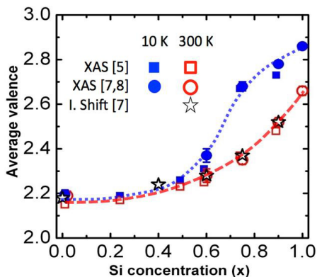
Fig. 2. Concentration dependence of the average valence derived from L_3 -edge X-ray spectroscopy [from Refs. Fukuda et al. (2003) (squares) and Alekseev et al. (2014), Alekseev et al. (2012) (circles)] and Mössbauer isomer shift [from Ref Alekseev et al. (2014) (stars)]. Open (closed) symbols denote values for T = 300 K (10 K). Lines are guides to the eye.
