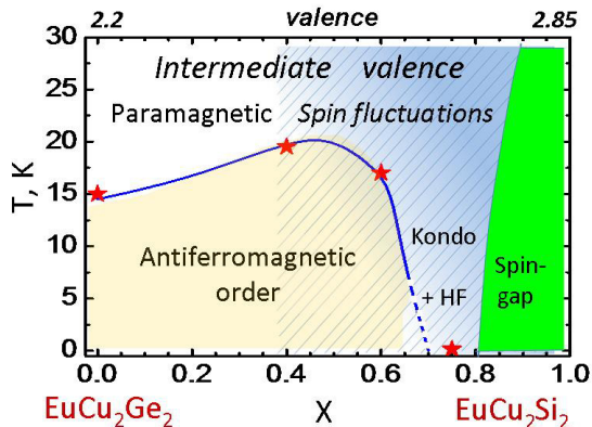
Fig. 3. Magnetic phase diagram of \text{EuCu}_2(\text{Si}_x\text{Ge}_{1-x})_2 . The solid blue line separating the paramagnetic and LRMO regions represents the results of Ref. Hossain et al. (2004). Stars indicate T_N values obtained our neutron diffraction study Alekseev et al. (2014). The green-colored area corresponds to the spin-gap regime, and the hatched area to the spin-fluctuation regime, in which a QE response is experimentally observed. A Kondo + HF region exists, according to Ref. Hossain et al. (2004), in between the spin-gap and LRMO states.
