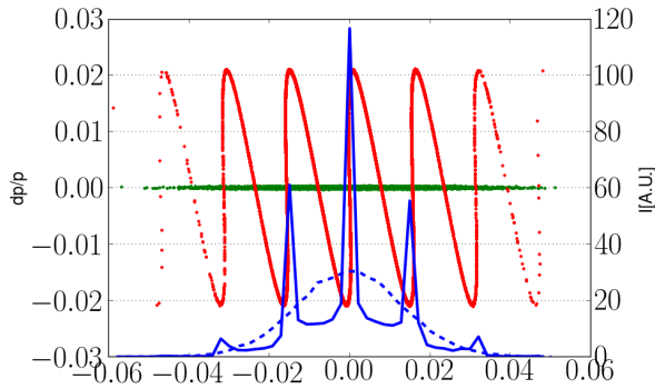
Figure 3: Simulated longitudinal phase space at the entrance (green) and after the bunch compressor (red) with 12 GHz cavity. Current profiles before (blue dashed line) and after (solid blue line) are shown.
