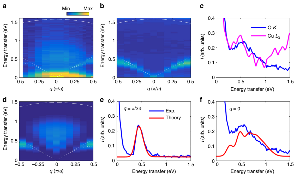
Fig. 2 Comparison between the experimental and calculated RIXS spectra at the oxygen K-edge. a, b Experimental RIXS spectra as a function of momentum transfer and energy transfer measured at the oxygen K-edge with an incident photon energy of \hbar\omega_{in} = 528.6 eV (resonance B) ( a ) and at the copper L_3 -edge from ref. 4 ( b ). c compares the O K-edge (blue) and Cu L_3 -edge (magenta line) RIXS line cuts at q = 0 . In the case of Cu L_3 data, there is a tailing contribution from higher energy dd excitations, which extends down to low energy transfer (see Supplementary Note 3). d displays the calculated oxygen K-edge spectra for \hbar\omega_{in} = 500 meV. (This value optimizes the intensity of the four-spinon features, see Supplementary Note 5.) The excitation around 90 meV in the oxygen K-edge data is a phonon excitation not included in our model calculations. The modeled RIXS intensity was obtained from exactly diagonalizing a 22-site t - J chain with periodic boundary conditions and the elastic line has been removed from the data for clarity. e , and f show line cuts of the RIXS spectra at q = \pi/2a and q = 0 , respectively. The experimental (theoretical) data are represented by the blue (red) solid lines. The intensity of the RIXS data are reported in arbitrary units (arb. units). The dotted and dashed white lines in a , b , and d indicate the boundaries of the two- and four-spinon continua, respectively (for more details on these boundaries see Supplementary Note 4)
