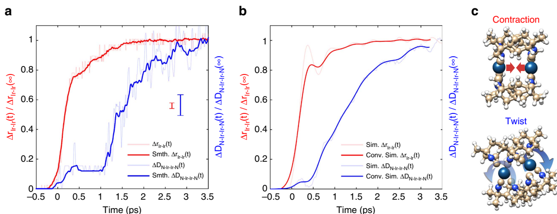
Figure 2 | Molecular structural dynamics of photoexcited [Ir_2(dimen)_4]^{2+} . (a) The Ir-Ir contraction (red) and the N-Ir-Ir-N dihedral twist (blue) determined from the XDS analysis. The full curves show the 15-point ( \sim 120 fs) smoothed result, with the parameter uncertainty being estimated by the point-to-point variation. Vertical lines show the average standard error at each time delay. (b) Ir-Ir contraction (red) and N-Ir-Ir-N dihedral twist (blue) determined from BOMD simulations (shaded lines) and the results from BOMD after convoluting the signal with the IRF of the experiment (full lines). (c) Schematic depiction of the contraction and twist distortions.
